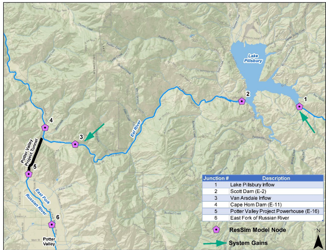
Figure 2: Schematic of Potter Valley Project ResSim Model
